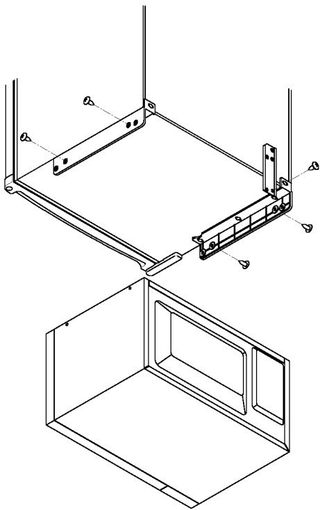
MicroFridge® with Safe Plug® Assembly Diagram - Model 3.6MF4RA
