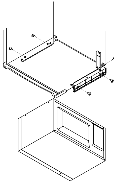
MicroFridge® Model MFRA-3 Assembly Diagram
