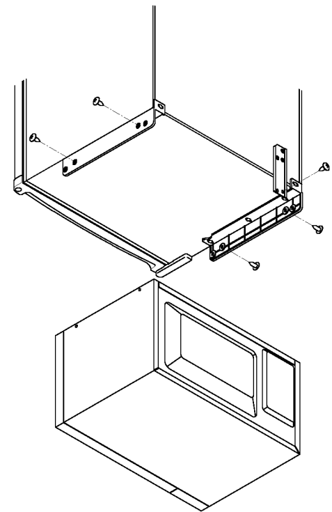
MicroFridge® with Safe Plug® Assembly Diagram - Model 3.0MF4R
